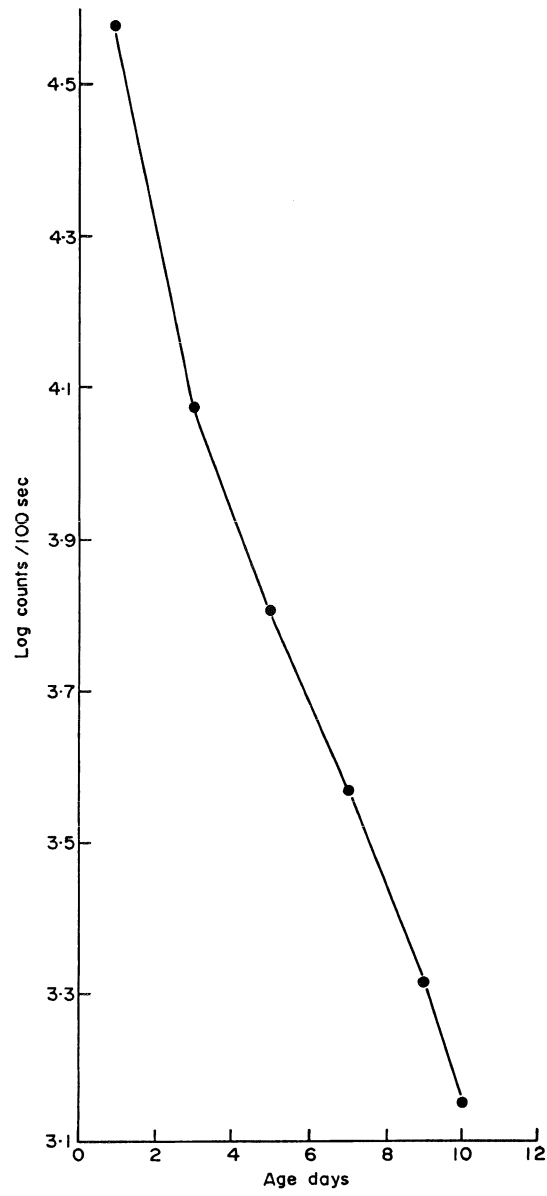
FIG. 2. The decrease with time of radioactivity (log counts/100 seconds) in plasma protein precipitates; pig P 11.
